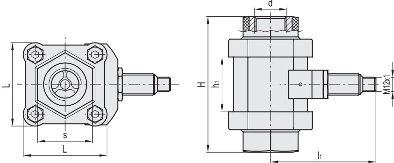
HVF-E (G3/4 - G1)
