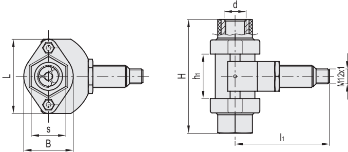
HVF-E (G3/8 - G1/2)
